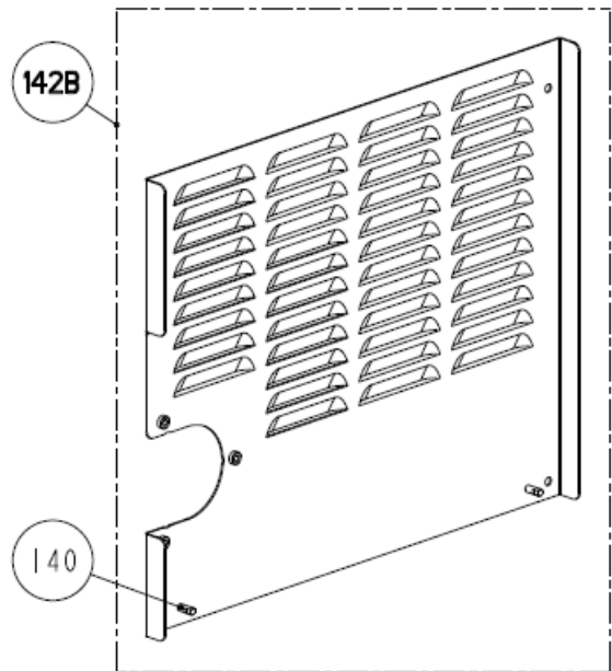
VENCLOSURE BELT SIDE PANEL (SIDEX)
