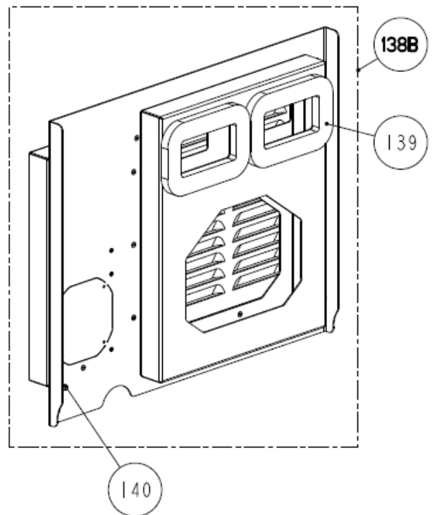
ENCLOSURE GENERATOR PANEL 5.0/4.2 MCGA
